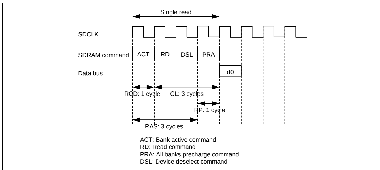
Figure 5 Read Timing
